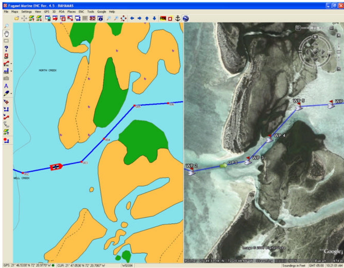
Fugawi Marine ENC with Google Earth Plug-in – Situational awareness of a poorly charted part of the Bahamas (left) is augmented by use of synchronized Google Earth Maps in split-screen mode (right). Sandbars, reefs and channels are more clearly identified.
